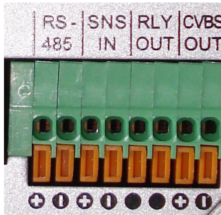
Figure 2-3 Terminal block for the I/O Connection of VSIP-2
