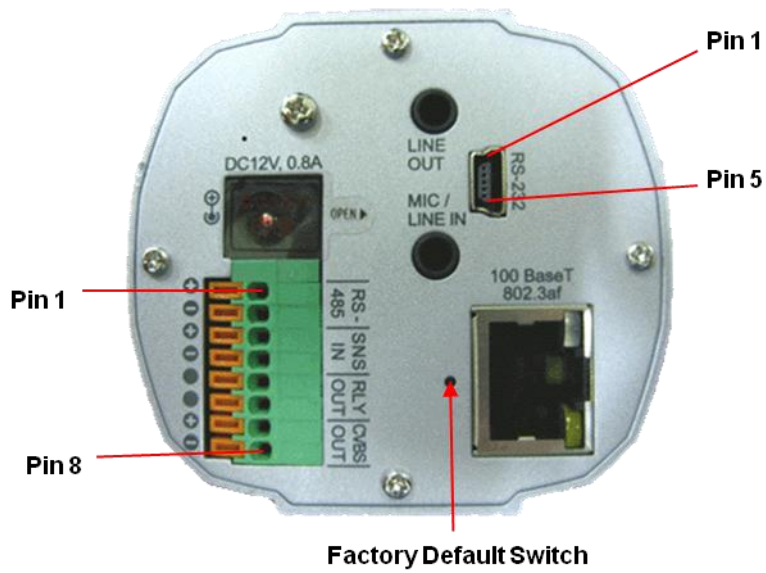
Figure 2-2. Rear panel of VSIP-2
